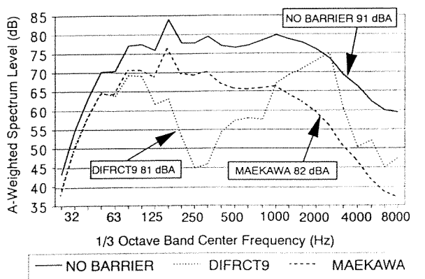
FIGURE 3 Boeing 727 departure spectrum at Site 1 with no barrier (measured) and a 6-m (20-ft) barrier.
